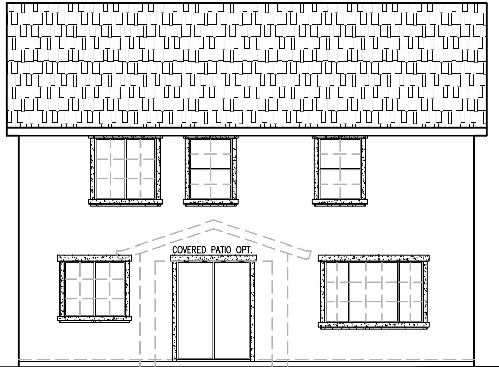
REAR ELEVATION 1/8" = 1'-0"
