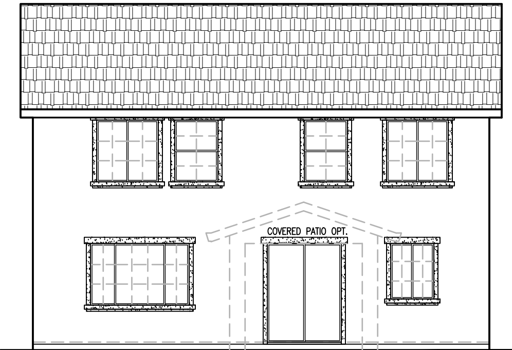
REAR ELEVATION 1/8" = 1'-0"
