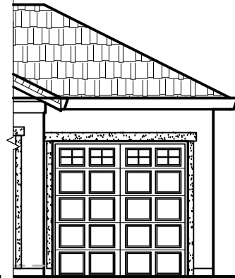
3 CAR GARAGE OPT. 1/8" = 1'-0"
