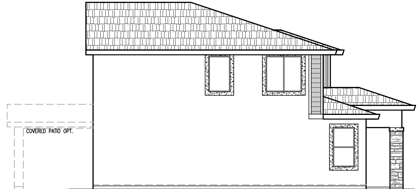
LEFT SIDE ELEVATION 1/8" = 1'-0"
