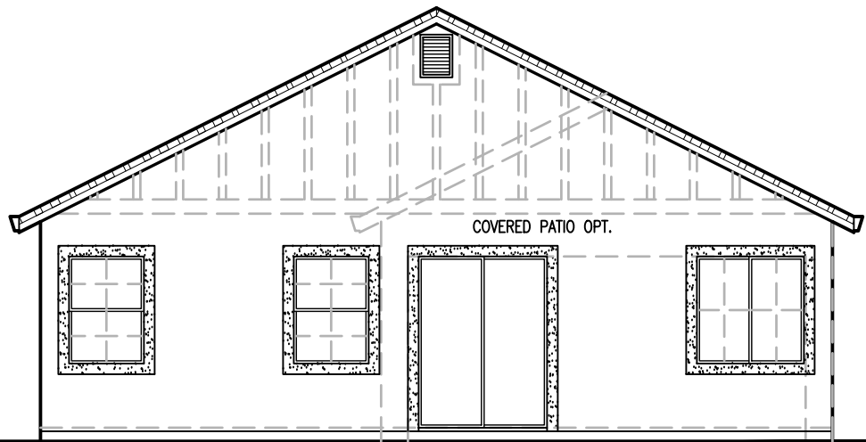
REAR ELEVATION 1/8" = 1'-0"
