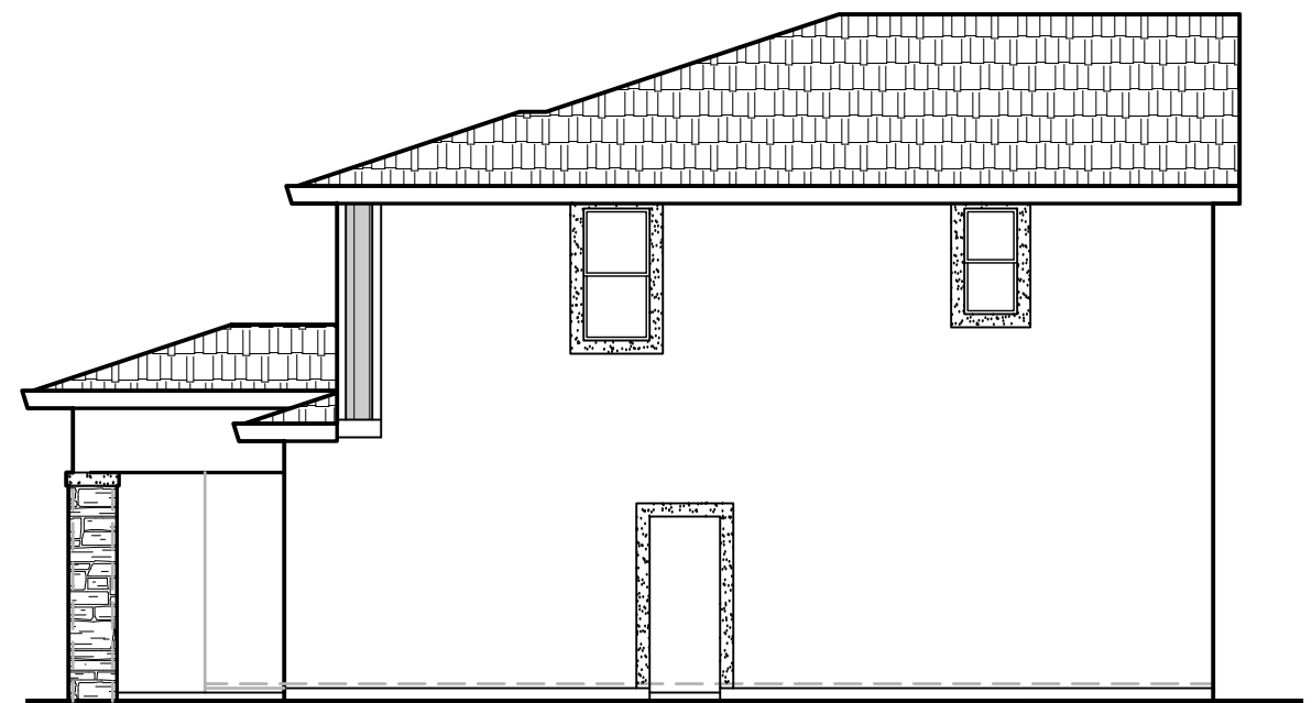
RIGHT SIDE ELEVATION 1/8" = 1'-0"
