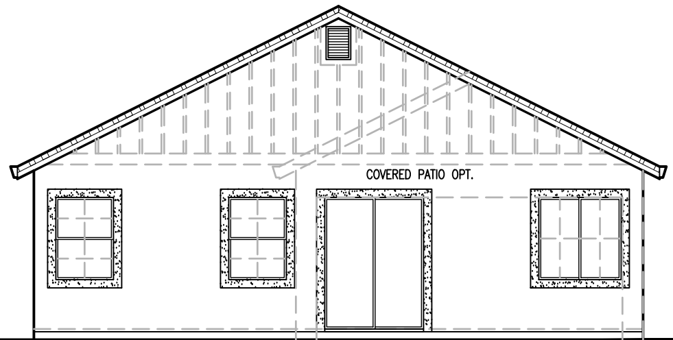
REAR ELEVATION 1/8" = 1'-0"
