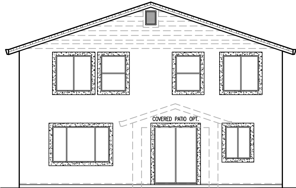
REAR ELEVATION 1/8" = 1'-0"
